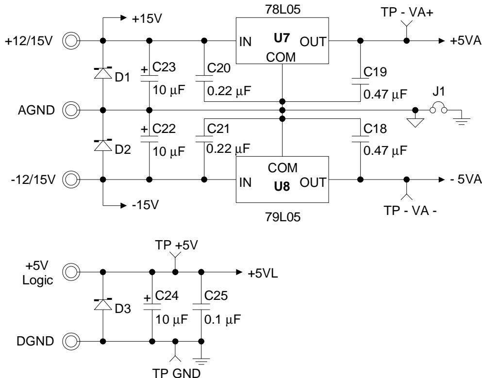
Figure 1. Power Supplies
