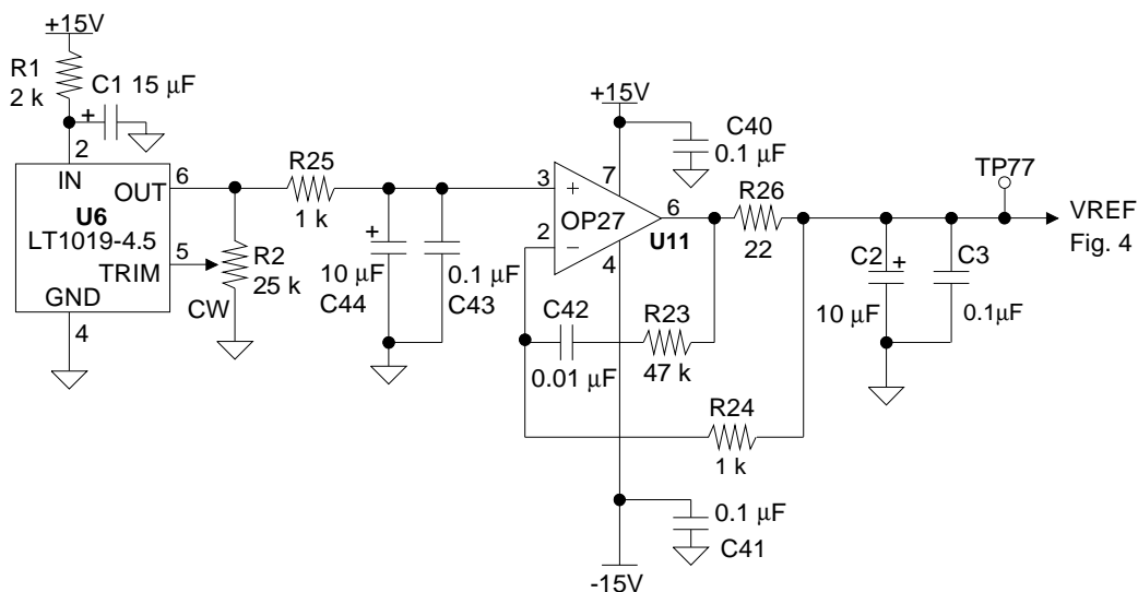
Figure 3. Voltage Reference
