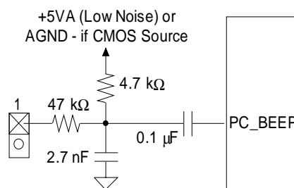
Figure 7. Mono Input
