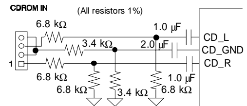
Figure 5. Differential CDROM In
