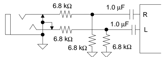
Figure 4. Line Inputs
