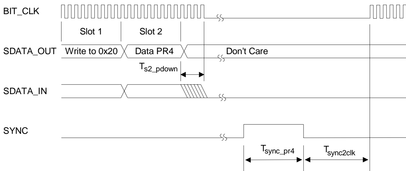
PR4 Powerdown and Warm Reset
