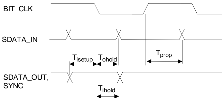
Data Setup and Hold
