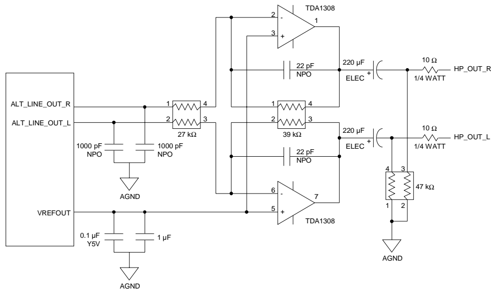
Figure 8. Headphones Driver
