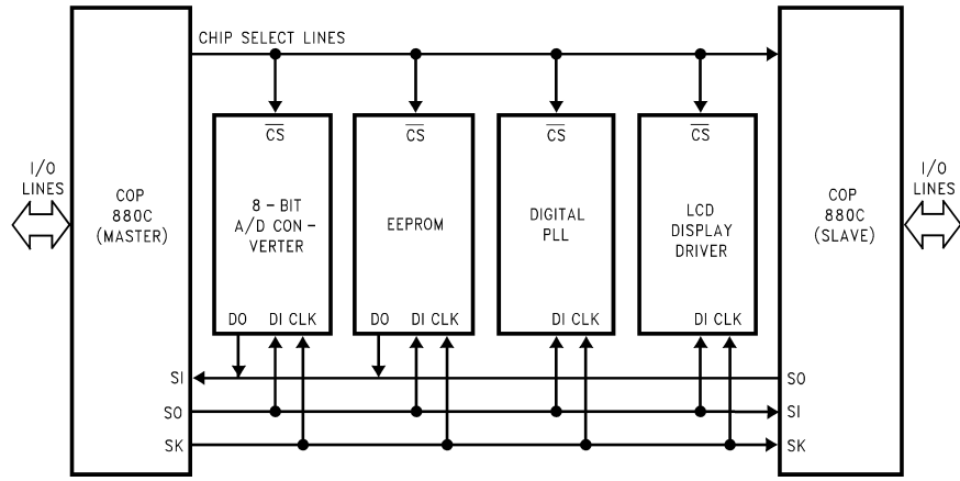
FIGURE 8. MICROWIRE/PLUS Application
