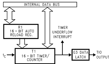
FIGURE 9. Timer/Counter Auto Reload Mode Block Diagram
