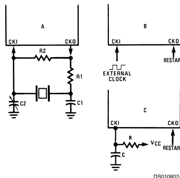
FIGURE 5. Crystal and R-C Connection Diagrams
