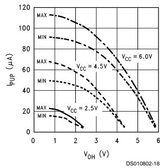
Port L/C/G Weak Pull-Up
