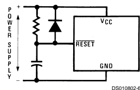
FIGURE 4. Recommended Reset Circuit
