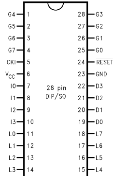
Dual-In-Line Package (N) and 28 Wide SO (WM)
