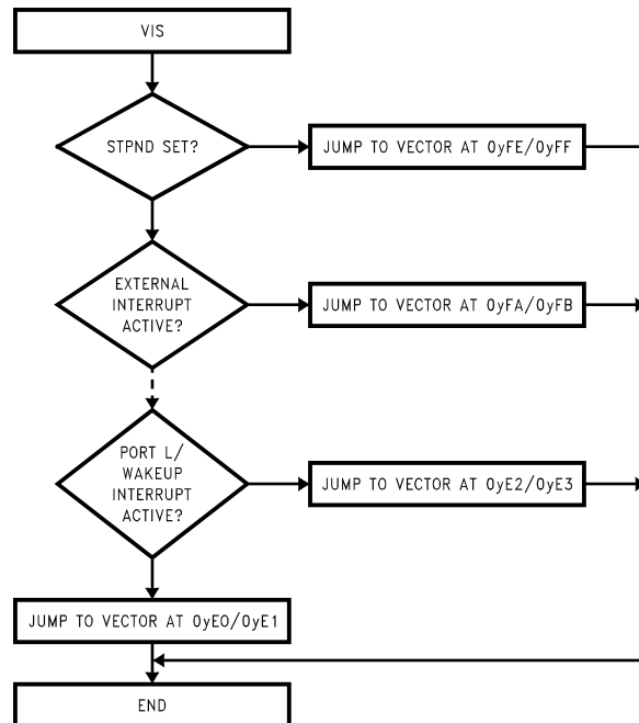
FIGURE 20. VIS Flowchart
