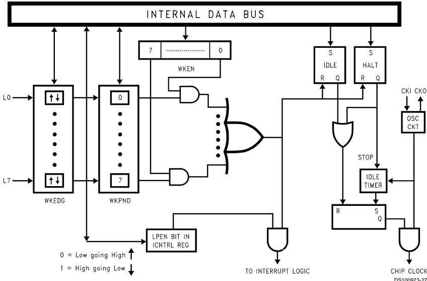
FIGURE 17. Multi-Input Wake Up Logic
