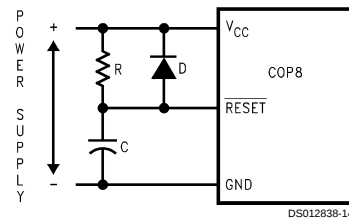
FIGURE 9. Reset Circuit Using External Reset
