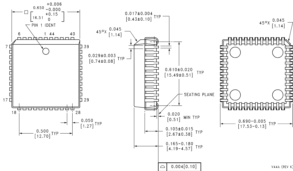
SLB package
