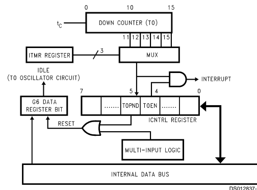
FIGURE 8. Functional Block Diagram for Idle Timer T0
