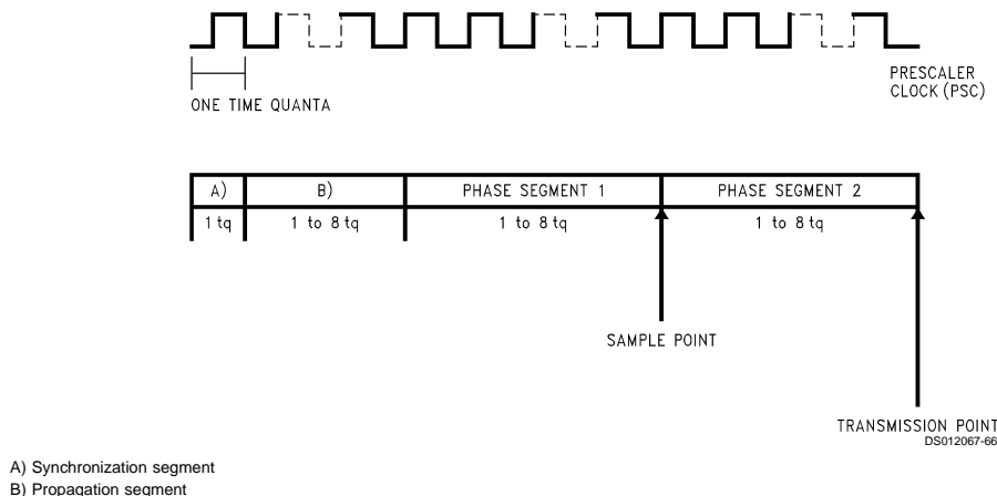
FIGURE 31. Bit Timing
