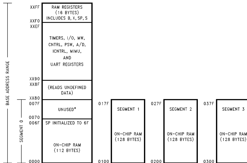
FIGURE 5. RAM Organization
