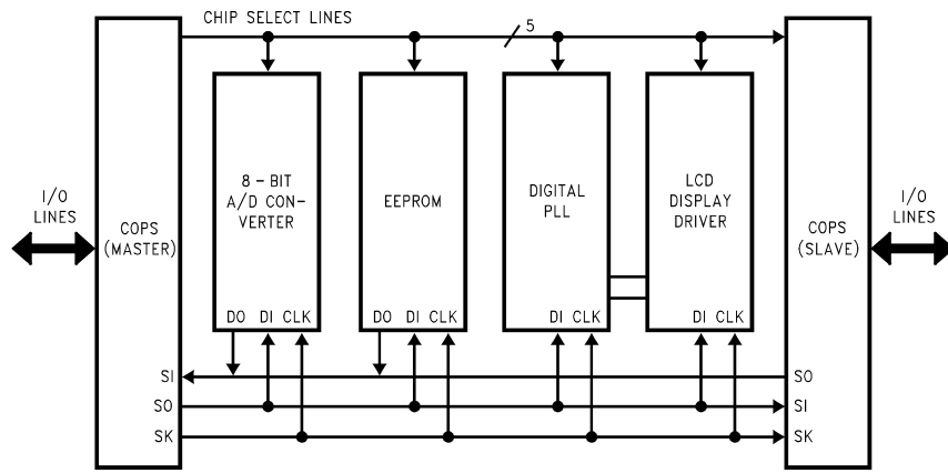
FIGURE 20. MICROWIRE/PLUS Application
