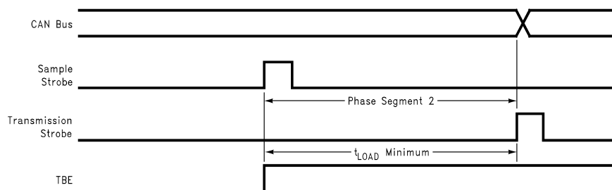
FIGURE 16. TBE Timing
