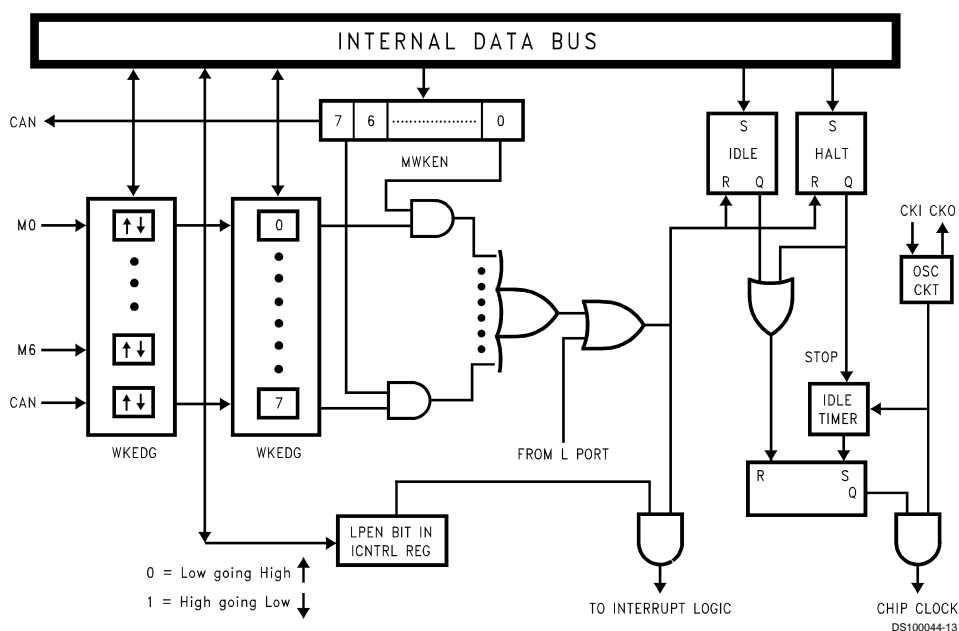
FIGURE 12. Port M Multi-Input Wake-up Logic
