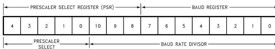
FIGURE 47. USART BAUD Clock Divisor Registers
