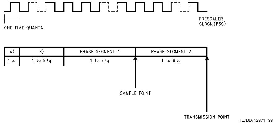
FIGURE 29. Bit Timing
