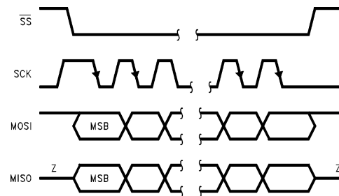
FIGURE 39. Slave Mode Communication
