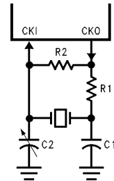
FIGURE 7. Crystal Oscillator Diagram
