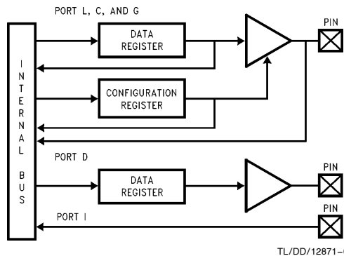
FIGURE 5. I/O Port Configurations
