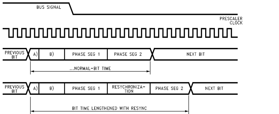
FIGURE 30. Resynchronization 1
