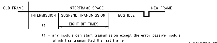
FIGURE 24. Interframe Space for Nodes Which Are Error Passive and Have Been Transmitter for the Last Frame
