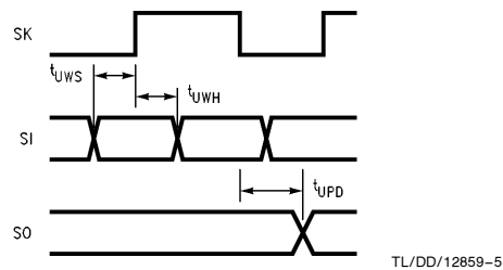
FIGURE 3. MICROWIRE/PLUS Timing
