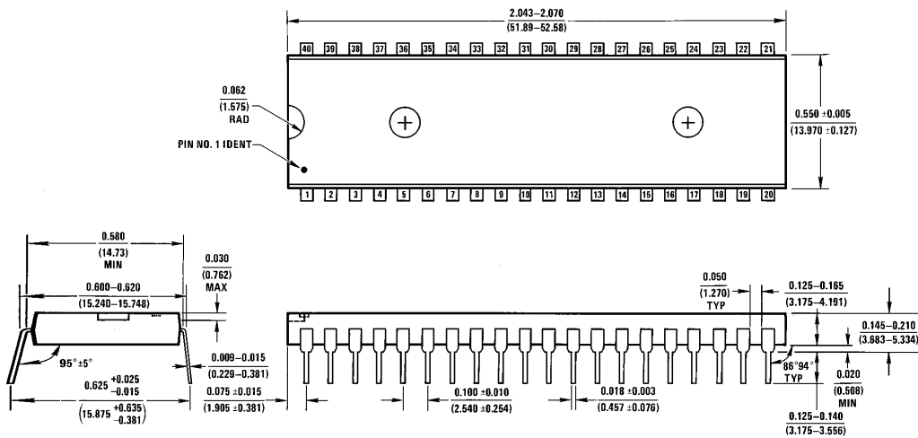
Molded Dual-In-Line Package (N) Order Number COP87L84RKN-XE NS Package Number N40A
