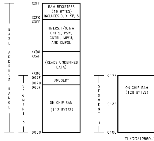
FIGURE 5. RAM Organization
