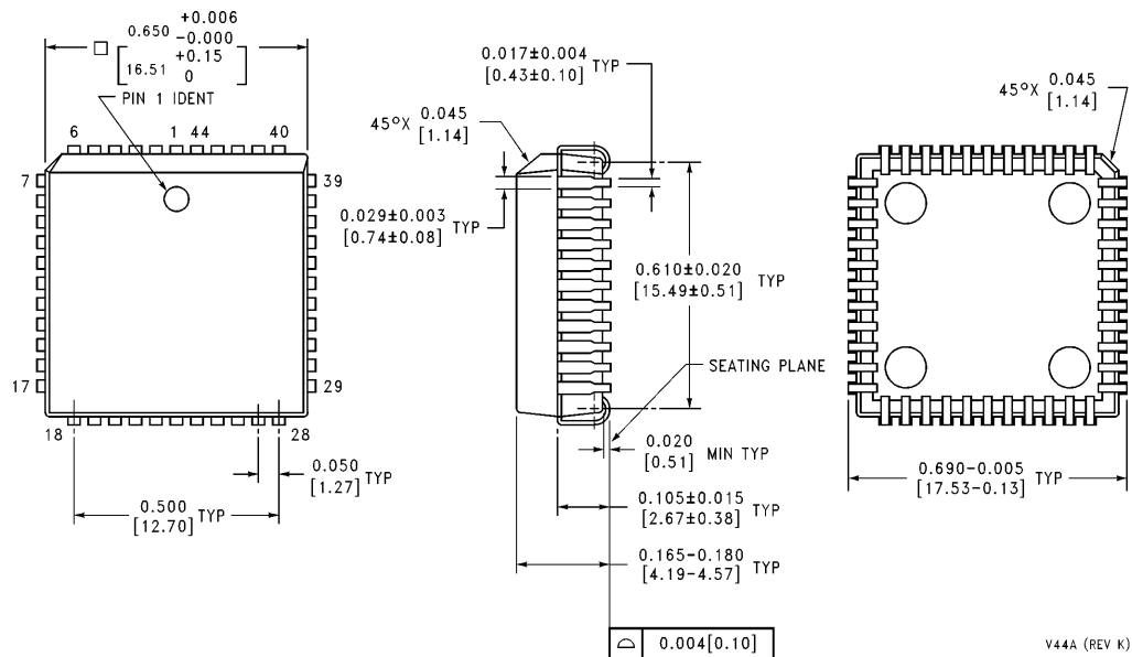
Plastic Leaded Chip Carrier (V) Order Number COP87L88RKV-XE NS Package Number V44A
