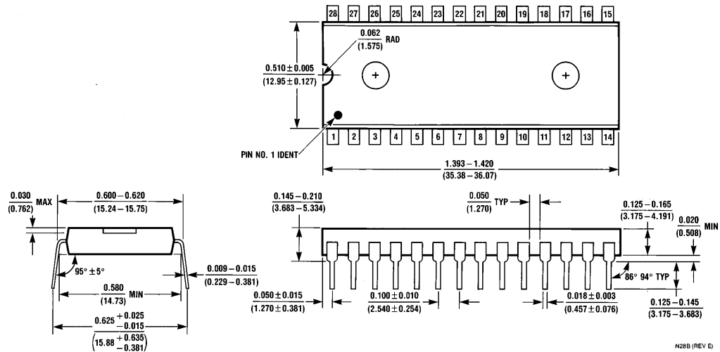
Molded Dual-In-Line Package (N) Order Number COP87L84RKN-XE NS Package Number N28B
