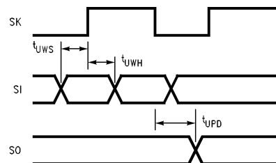
FIGURE 2. MICROWIRE/PLUS Timing
