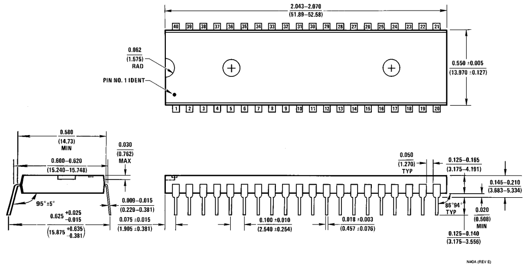
Molded Dual-In-Line Package (N) Order Number COP87L84CFN-XE NS Package Number N40A
