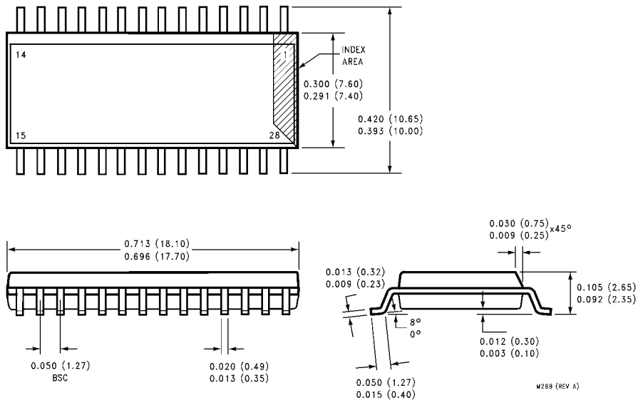
Molded SO Wide Body Package (M) Order Number COP87L84CFM-XE NS Package Number M28B
