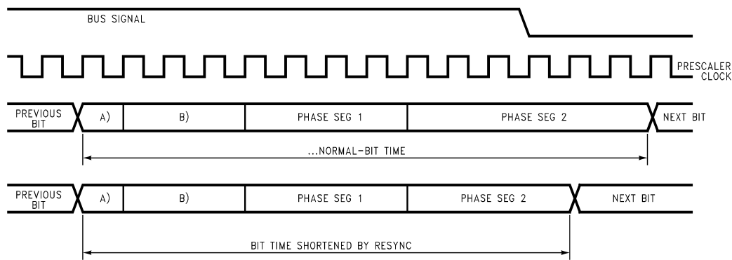
FIGURE 33. Resynchronization 2
