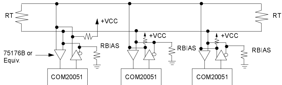
FIGURE 8 - COM20051+ NETWORK USING RS-485 DIFFERENTIAL TRANSCIEVERS
