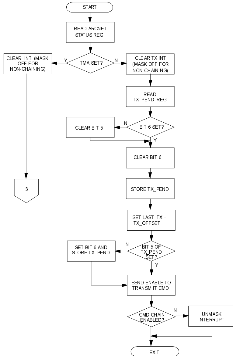
FIGURE 24 - TRANSMIT INTERRUPT SERVICE ROUTINE
