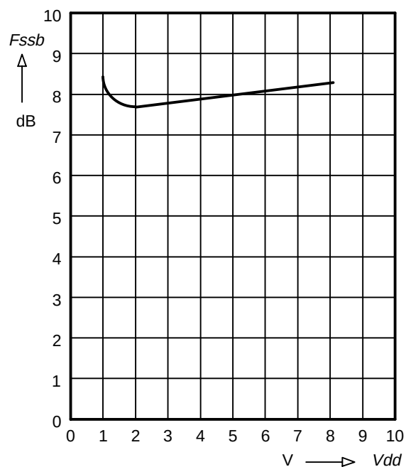
SSB Noise Figure F_{ssb} = f(V_{dd})
