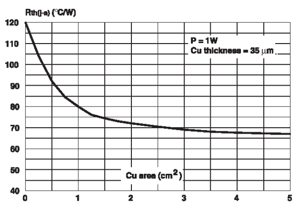
Fig. 2 : Junction to ambient thermal resistance versus copper surface under each lead.
