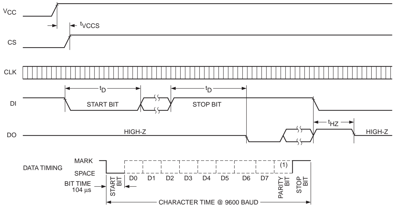
Figure 1. A.C. Timing
