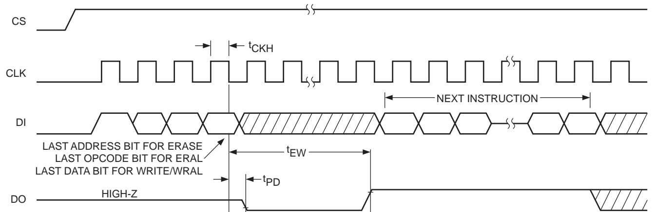
Figure 5. Program/Erase Timing
