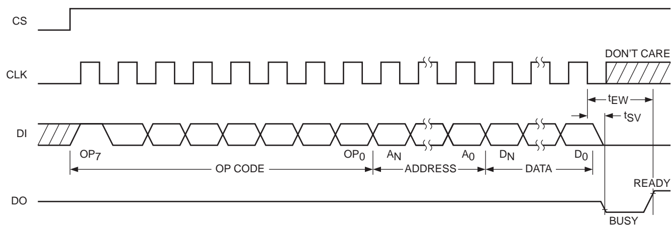
Figure 8. Write Timing
