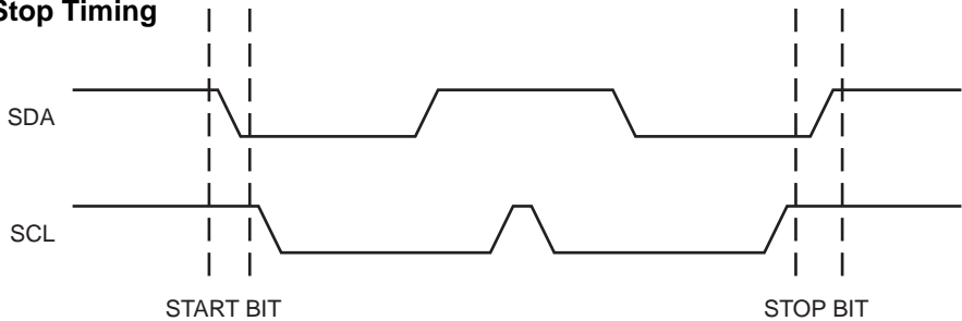
Figure 3. Start/Stop Timing
