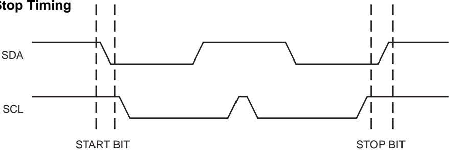
Figure 3. Start/Stop Timing
