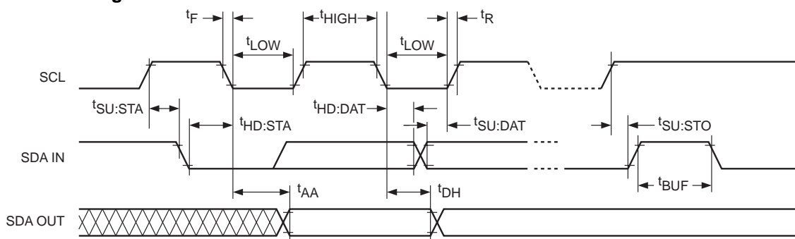
Figure 1. Bus Timing
