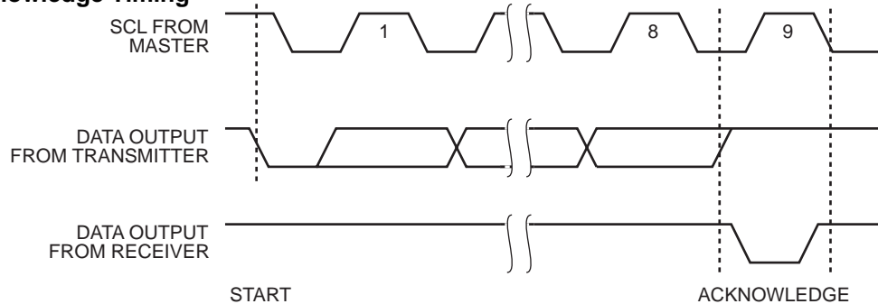
Figure 4. Acknowledge Timing
