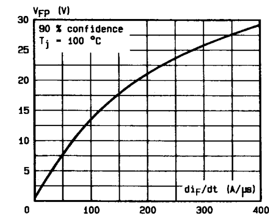
Figure 9. Peak forward voltage versus di_F/dt .
