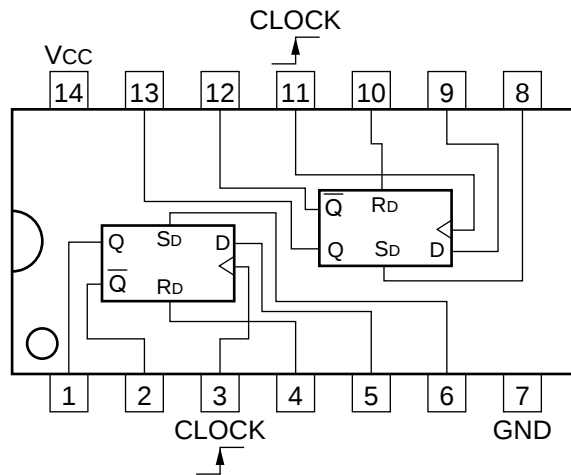
DIRECT R-S FLIP-FLOP
