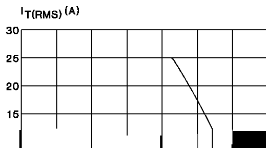
Fig.3 : RMS on-state current versus case temperature.
