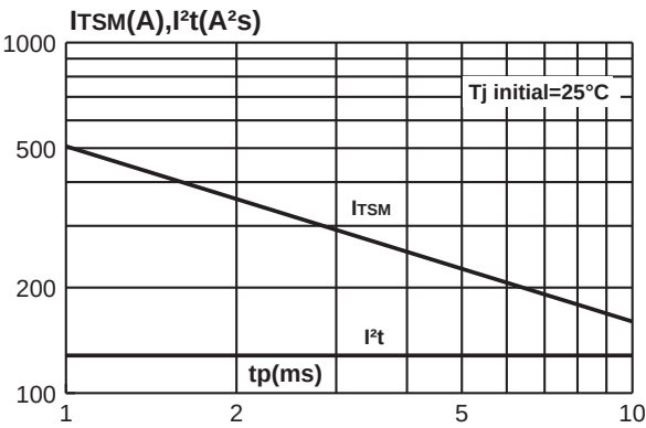
Fig 7 : Non repetitive surge peak on-state current for a sinusoidal pulse with width : t_p \leq 10 ms, and corresponding value of I^2t .
