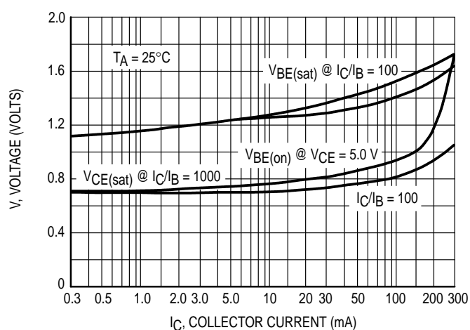
Figure 3. "On" Voltage
