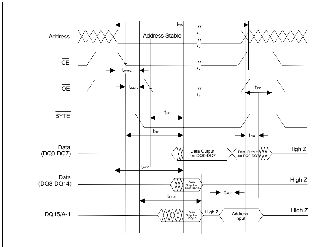
Figure 15. \overline{\text{BYTE}} Timing Diagram for Read Operation
