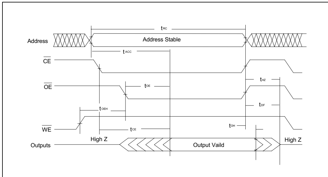
Figure 8. AC Waveforms for Read Operations
