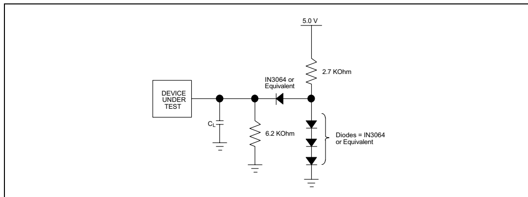
Figure 7. Test Condition
