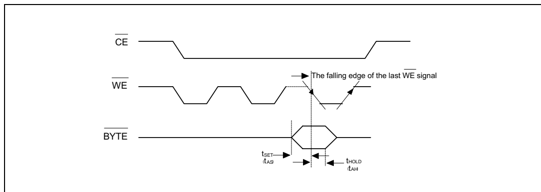
Figure 16. \overline{\text{BYTE}} Timing Diagram for Write Operation
