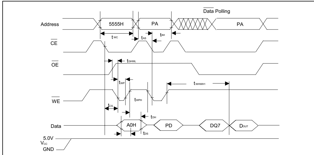
Figure 9. AC Waveforms Program Operations
