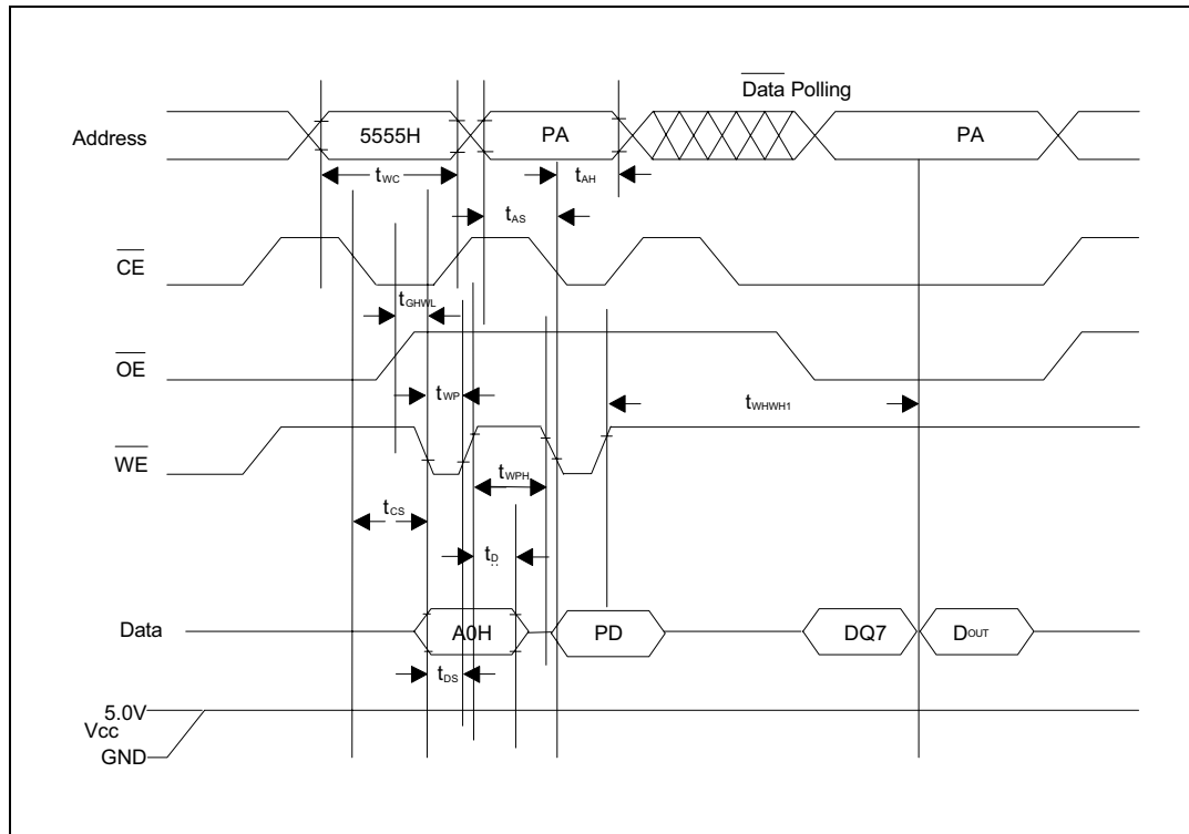
Figure 19. Alternate \overline{\text{CE}} Controlled Program Operation Timings
