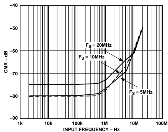
Figure 45. CMR vs. Input Frequency ( V_{CML} = 2 V p-p, 1× Mode)
