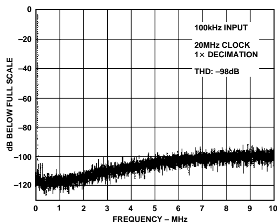
Figure 8. Spectral Plot of the AD9260 at 100 kHz Input, 20 MHz Clock, Undecimated (20 MHz Output Data Rate)
