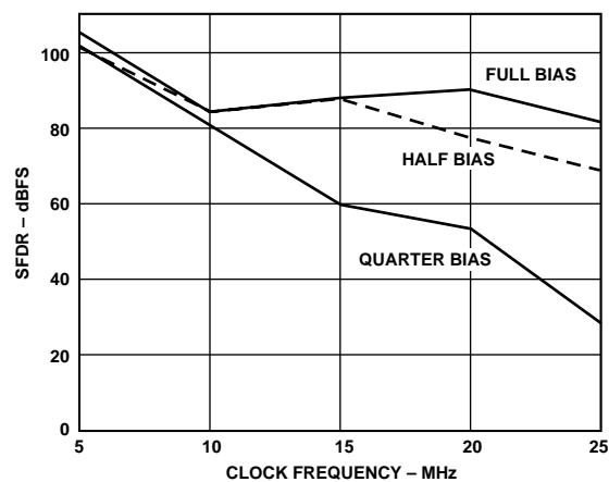
Figure 42. SFDR vs. Clock Rate ( f_{IN} = 500 kHz in 4× Mode)
