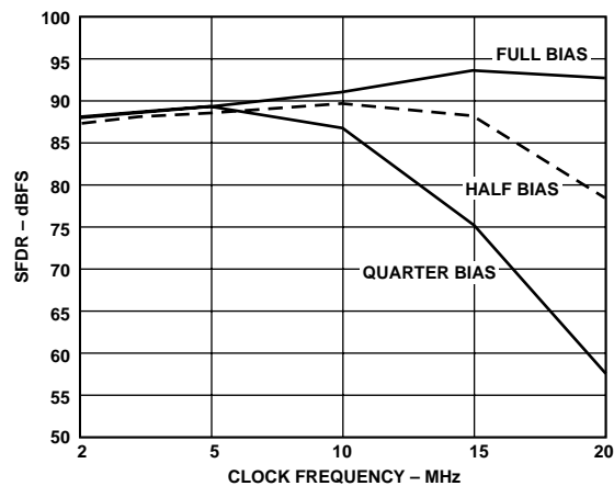
Figure 41. SFDR vs. Clock Rate ( f_{IN} = 100 kHz in 8× Mode)
