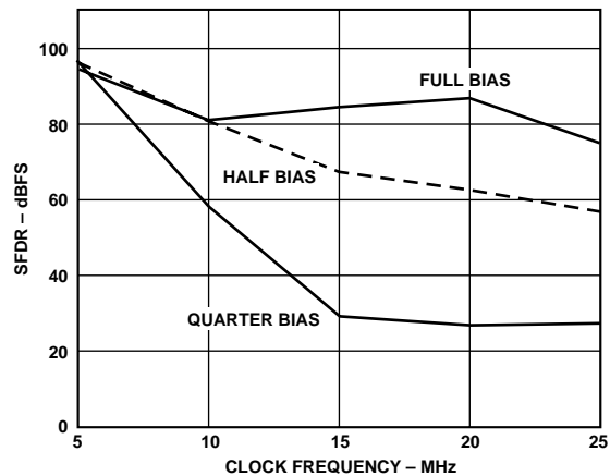
Figure 43. SFDR vs. Clock Rate ( f_{IN} = 1.0 MHz in 2× Mode)
