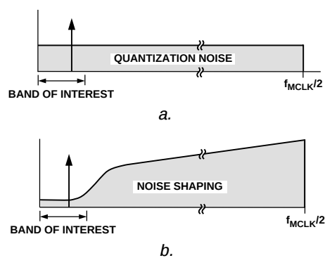
Figure 21. Sigma-Delta ADC
