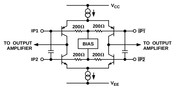
Figure 13. Equivalent Input Circuit
