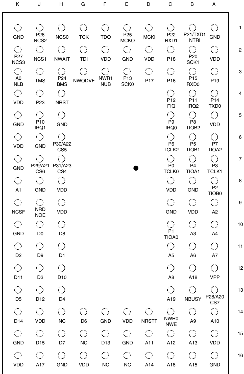
Figure 1. AT91FR4081 Pinout for 120-ball BGA Package (Top View)
