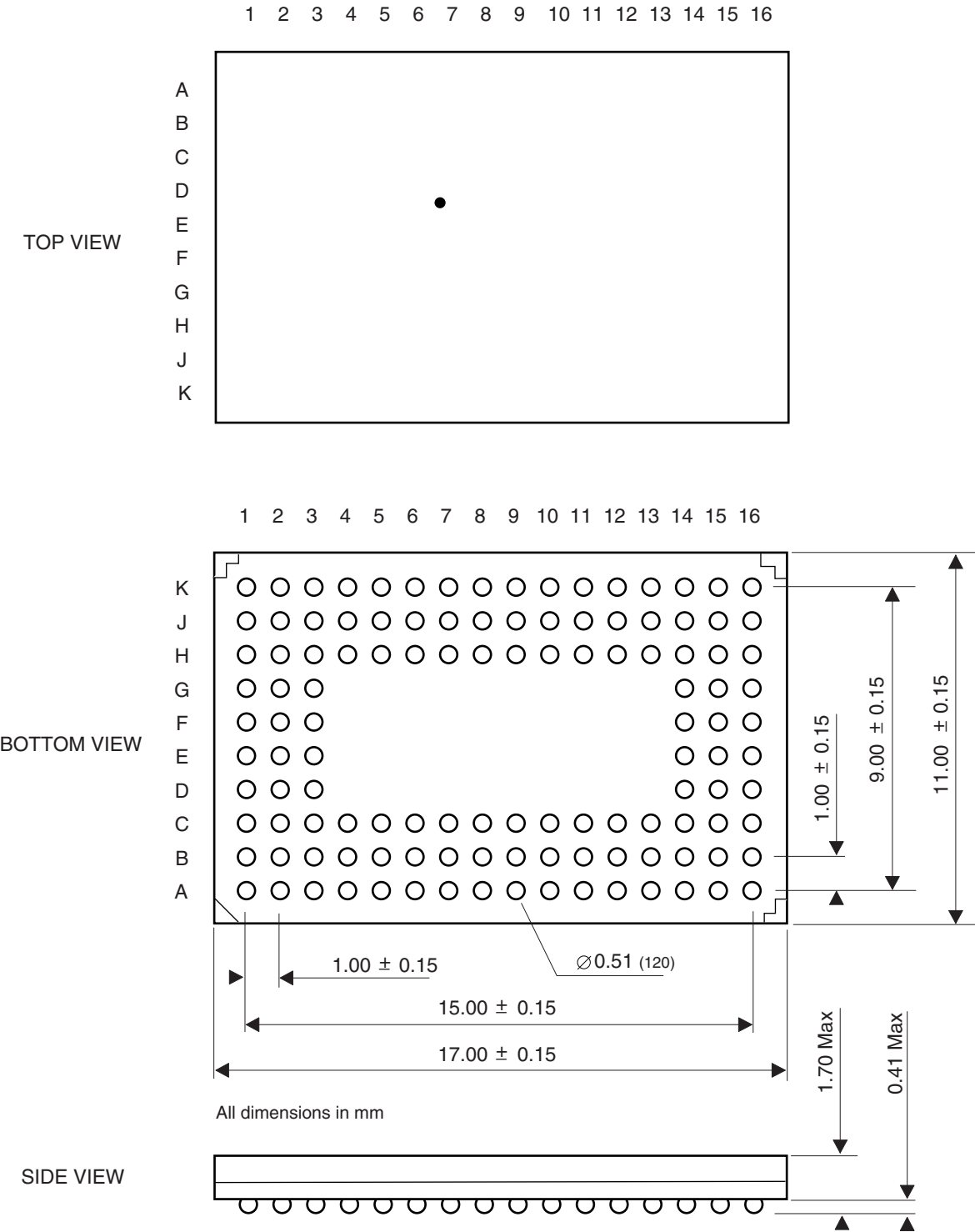
Figure 2. 120-ball BGA Package
