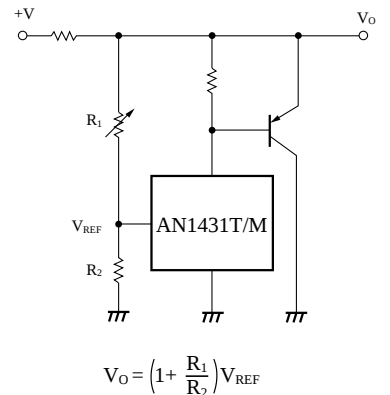
4.Current Boost
