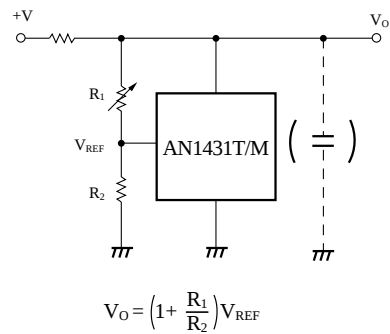
1.Shunt Regulator
