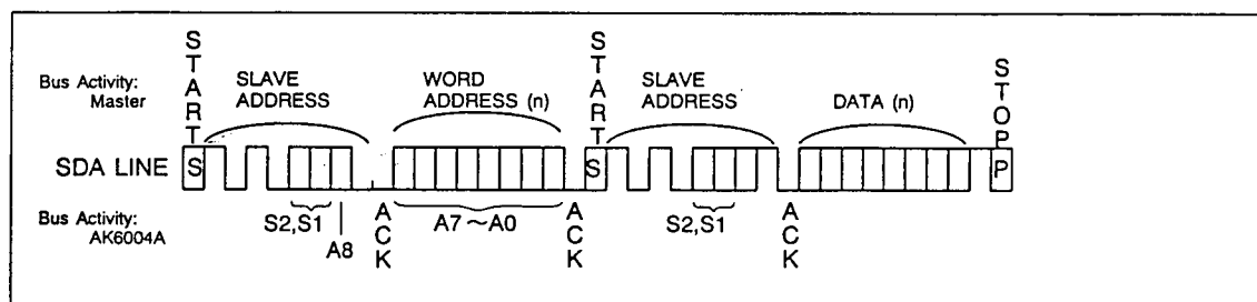
RANDOM READ
