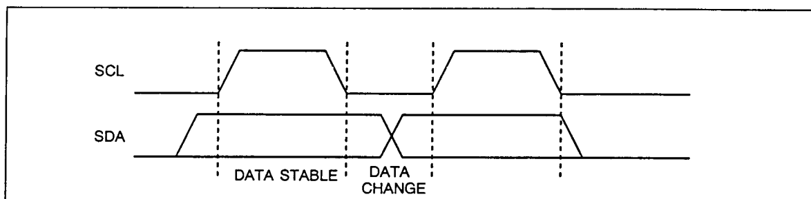
Figure1. Data transfer
