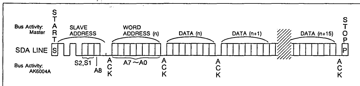
PAGE WRITE
