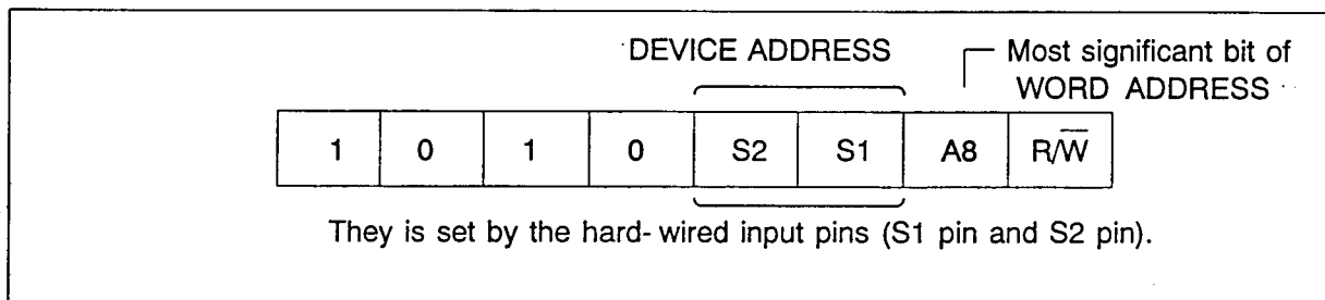
Figure4. Slave Address
