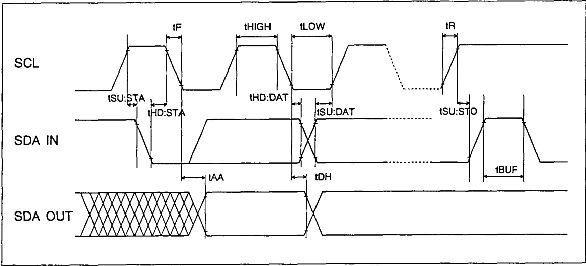
BUS TIMING
