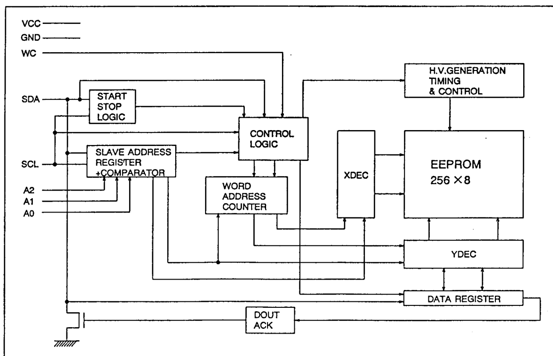
Block Diagram
