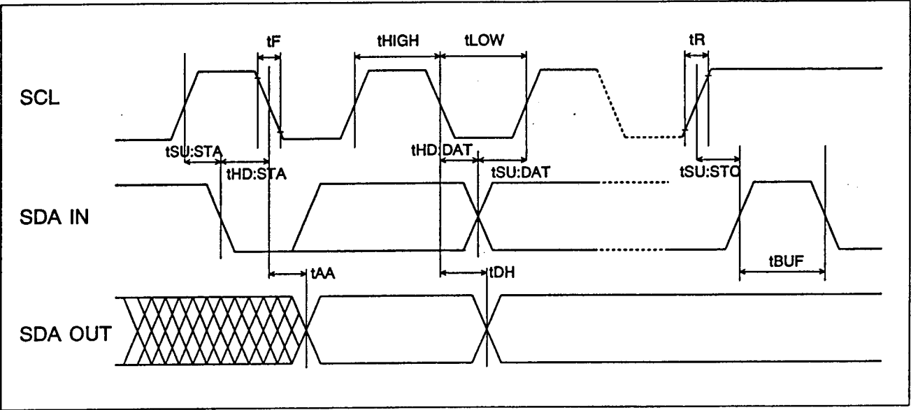
BUS TIMING
