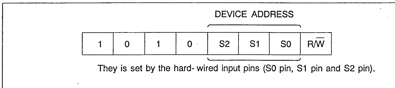
Figure4. Slave Address
