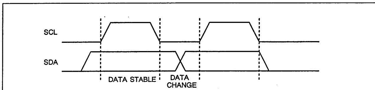
Figure1. Data transfer
