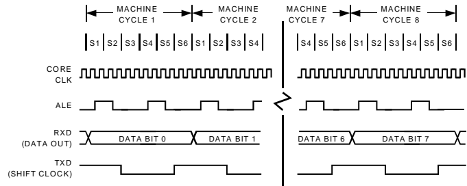
Figure 50. UART Serial Port Transmission, Mode 0.
