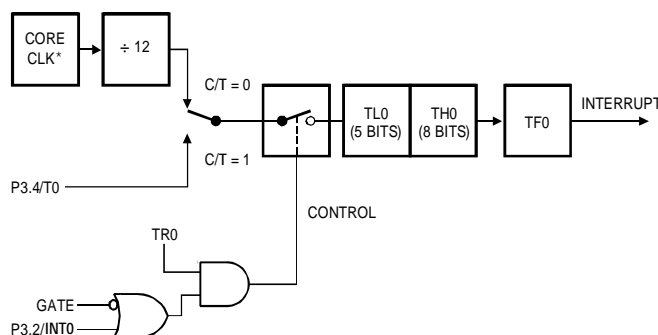
Figure 44. Timer/Counter 0, Mode 0
