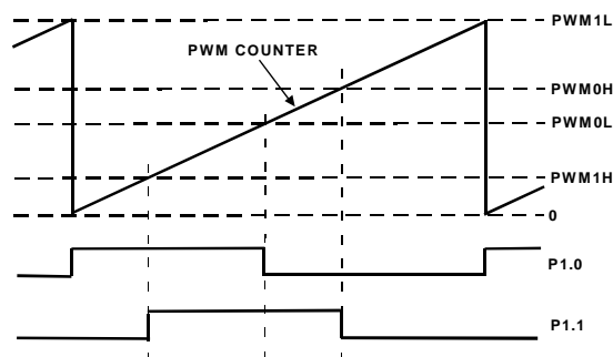
Figure 37. PWM Mode 2
