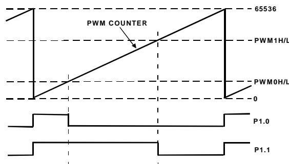
Figure 38. PWM Mode 3
