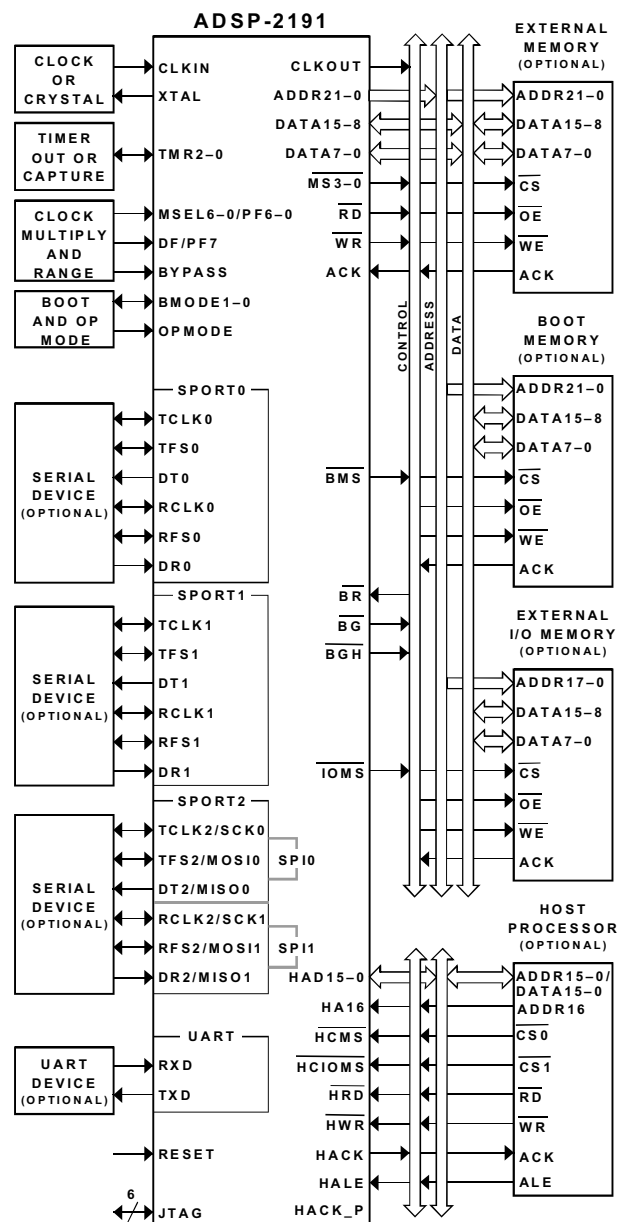
Figure 1. ADSP-2191 System Diagram
