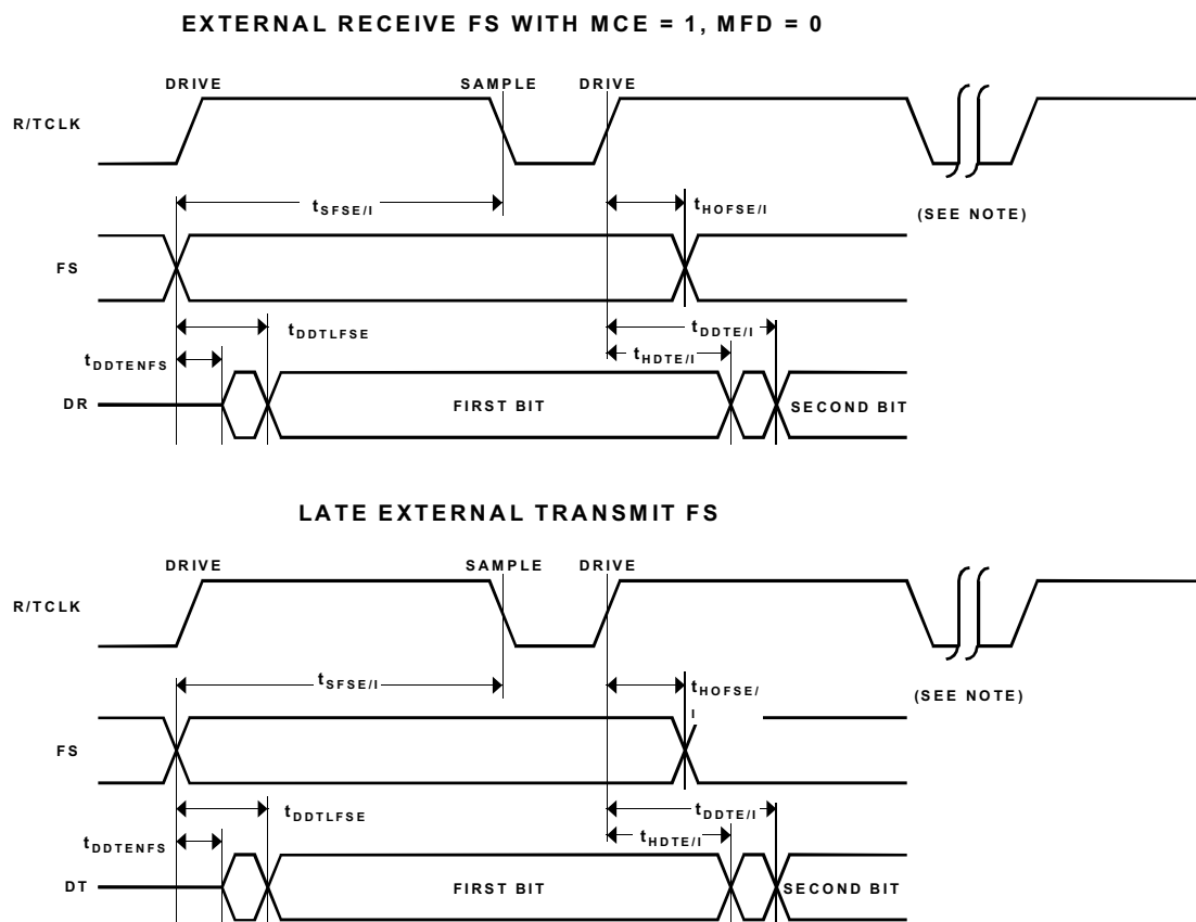
Figure 21. Serial Port (SPORT) Frame Sync
