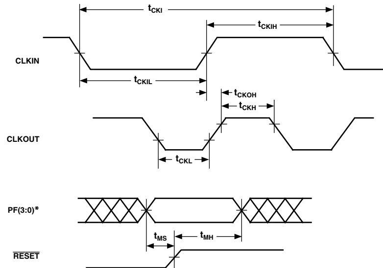
Figure 21. Clock Signals
