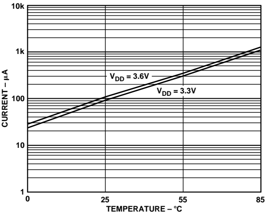
Figure 29. Power-Down Graph
