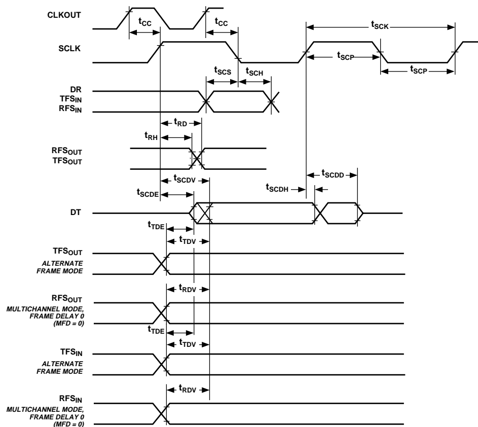
Figure 16. Serial Ports
