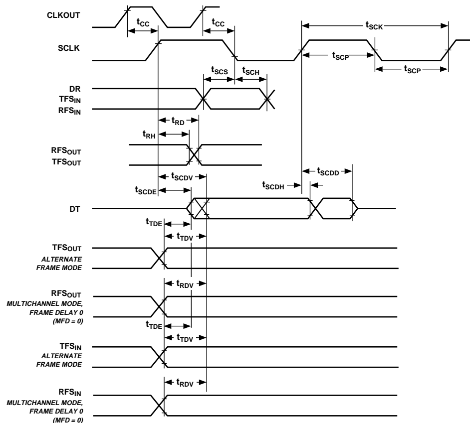
Figure 16. Serial Ports
