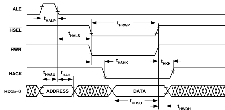
Host Write Cycle
