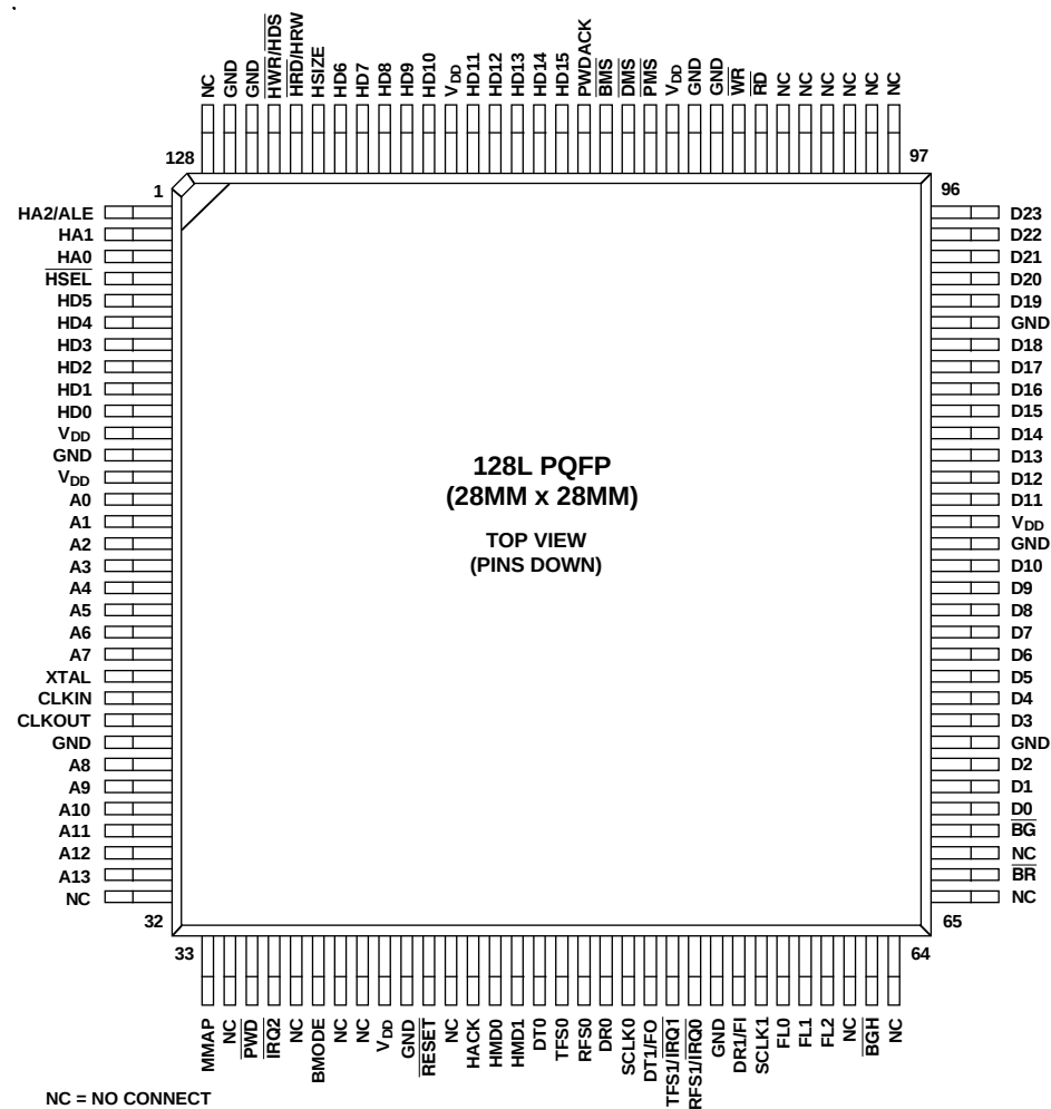
128-Lead PQFP Package Pinout
