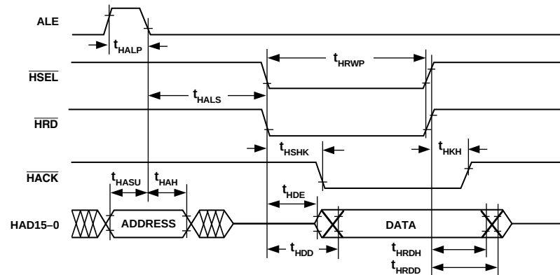
Figure 16. Host Interface Port (HMD1 = 1, HMD0 = 0)
