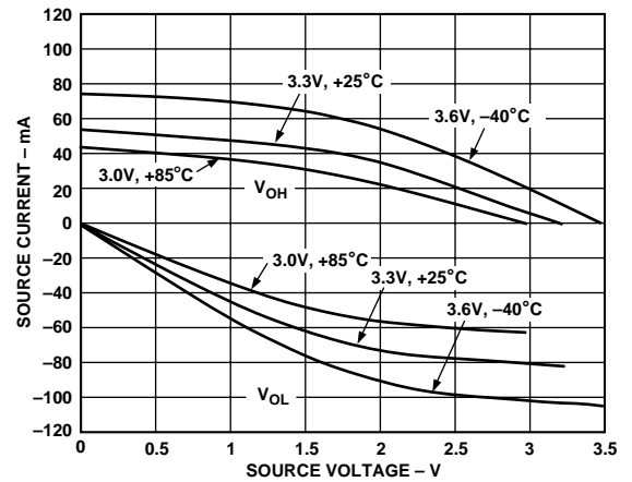
Figure 32. ADSP-2106x Typical Drive Currents ( V_{DD} = 3.3\text{ V} )
