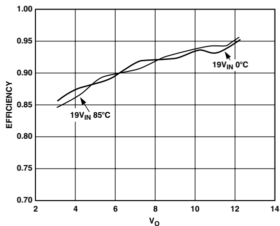
TPC 15. Conversion Efficiency vs. Battery Voltage at Temperatures
