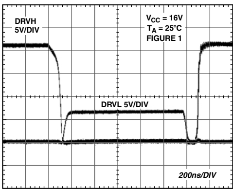
TPC 12. Driver Waveforms
