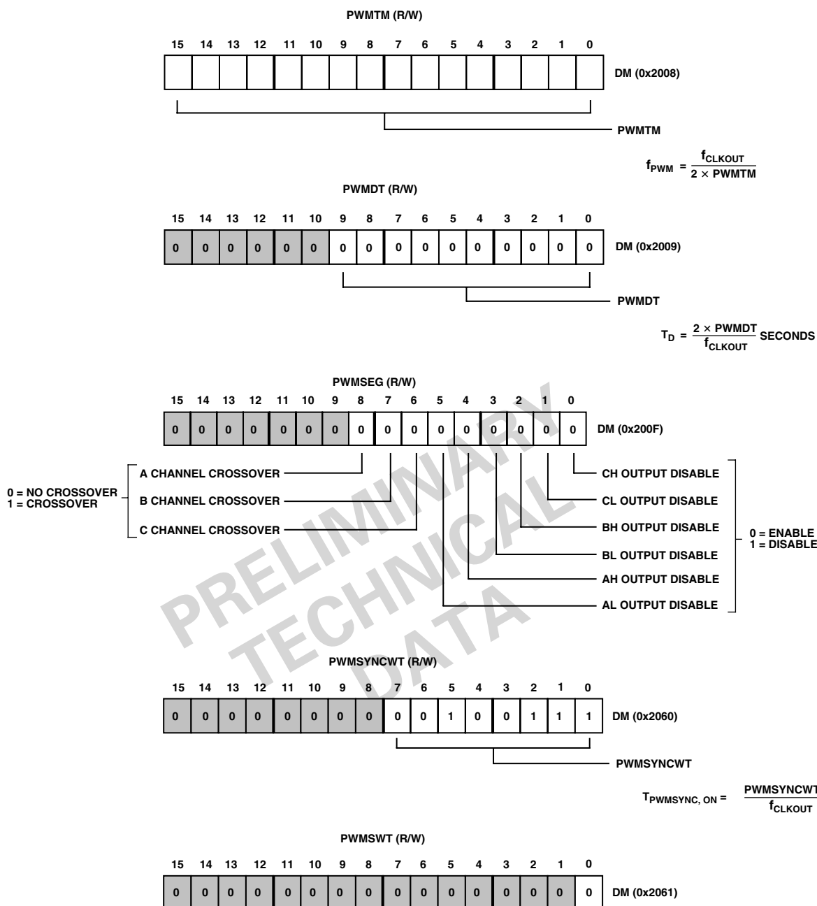
Figure 22. Configuration of PWM Registers
