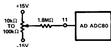
Figure 7. Offset Adjustment Circuit
