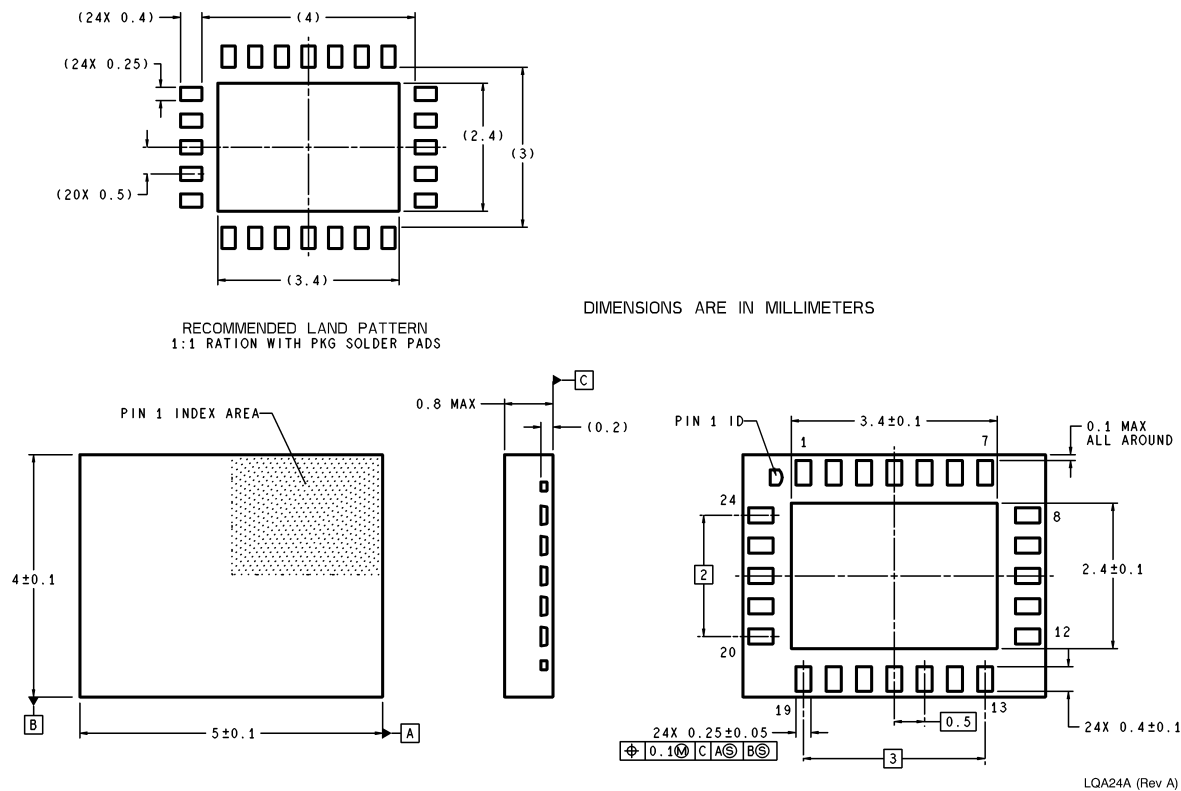
24-Lead Package LLP Order Number ADC08351CILQX NS Package Number LQA24A
