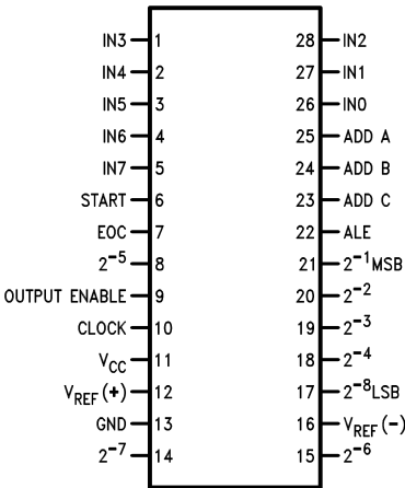
Dual-In-Line Package
