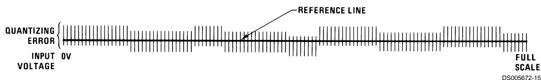
FIGURE 4. Typical Error Curve
