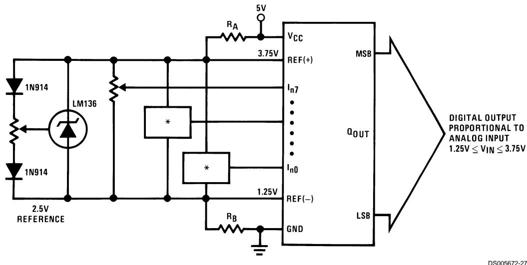
FIGURE 12. Typical Reference and Supply Circuit
