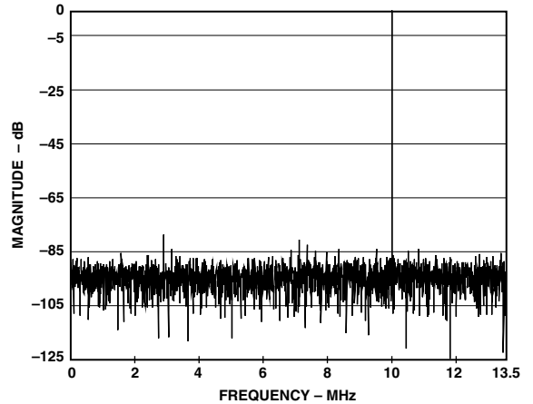
TPC 25. 10-Bit ADC Single-Tone Spectral Plot Without PLL (Input Frequency = 10 MHz, 4096 Point FFT)
