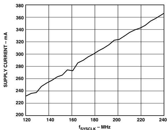
TPC 1. Power Consumption vs. Clock Speed, f_{SYSCLK}
