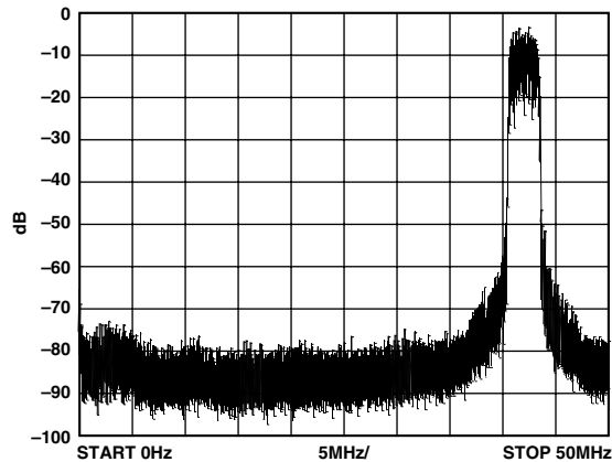
Figure 1. QPSK at 42 MHz and 2.56 MS/s; 10.24 MHz External Clock with REFCLK Multiplier = 12, CIC Interpolation Rate = 3, 4× Oversampled Data
