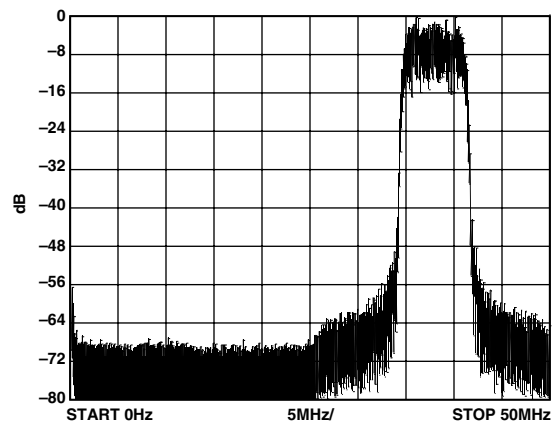
Figure 4. 256-QAM at 38 MHz and 6 MS/s; 48 MHz External Clock with REFCLK Multiplier = 4, CIC Interpolation Rate = 2, 4× Oversampled Data
